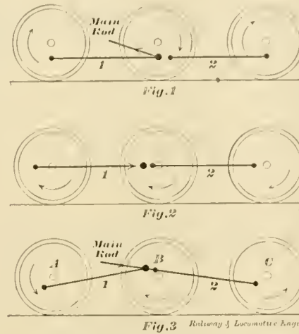
DISCONNECTING COUPLED RODS.
